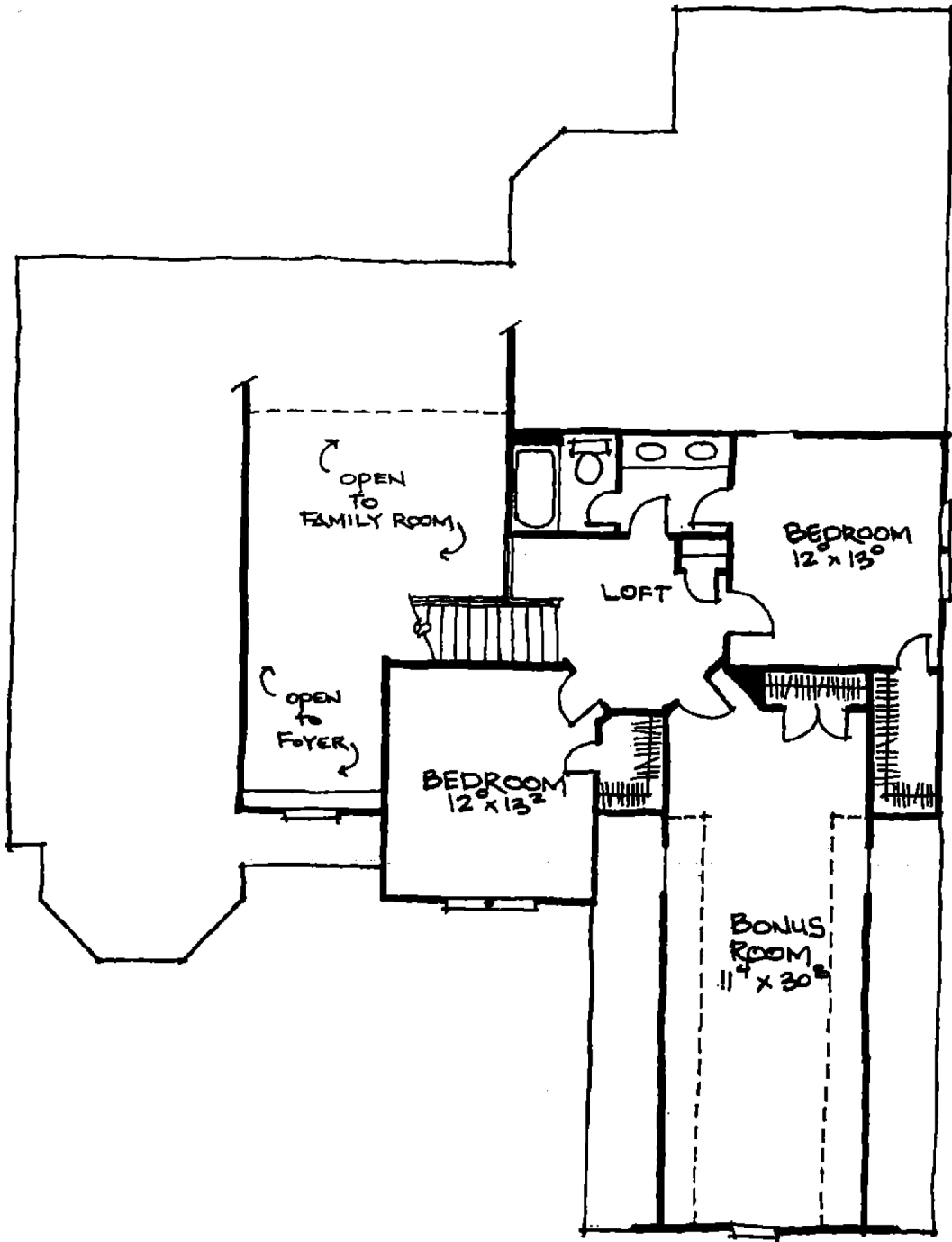
SECOND FLOOR PLAN ± 973 HEATED SQ. FT.
